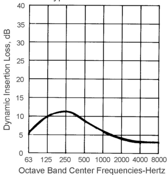
Typical Performance
