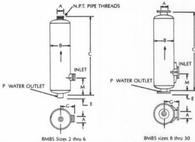
BMBS Sizes 2 thru 6
